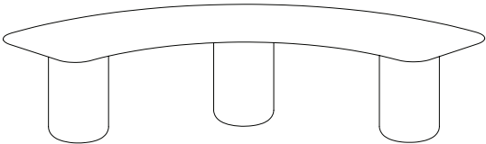
Curved Bench Large Size: 200cm x 74cm — Approx. 45kg Small Size: 166cm x 64cm — Approx. 40kg 25cm Ø Legs 42cm H Fitted upholstered cushions available on request
